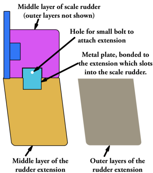
Figure A Constructing a rudder extension.
