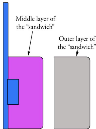
Figure F. Rudder construction using a small soldered "paddle"
